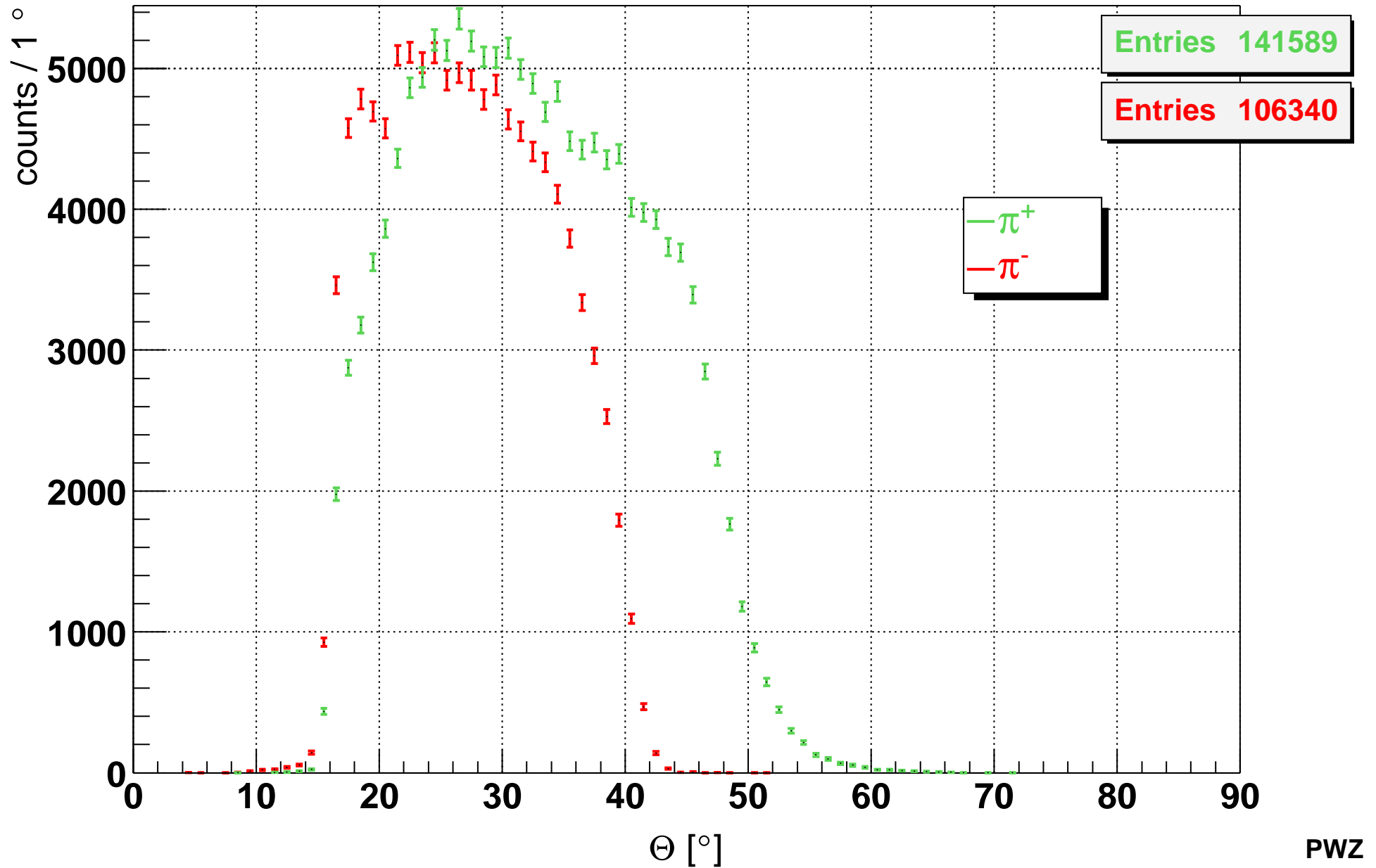
\ominus distribution of \pi^+ and \pi^- in system 0 (TOFino) -- NOV01-uncorrected
