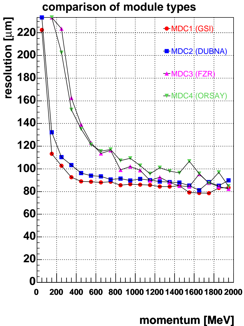
x position resolution vs momentum
