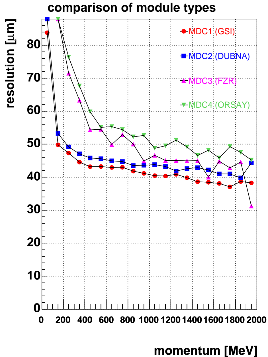
y position resolution vs momentum
