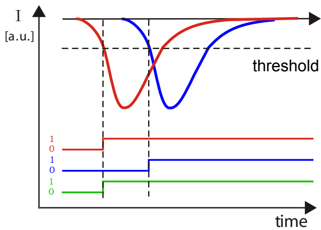
Two leading edges (TDC mode 1)
