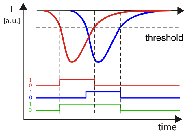
Leading and trailing edge (TDC mode 2)
